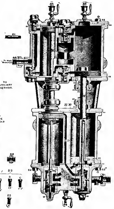
Fig. 1752. Duplex Air-pump.
